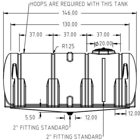
FM2350-88C CENTER DRAIN SUMP
