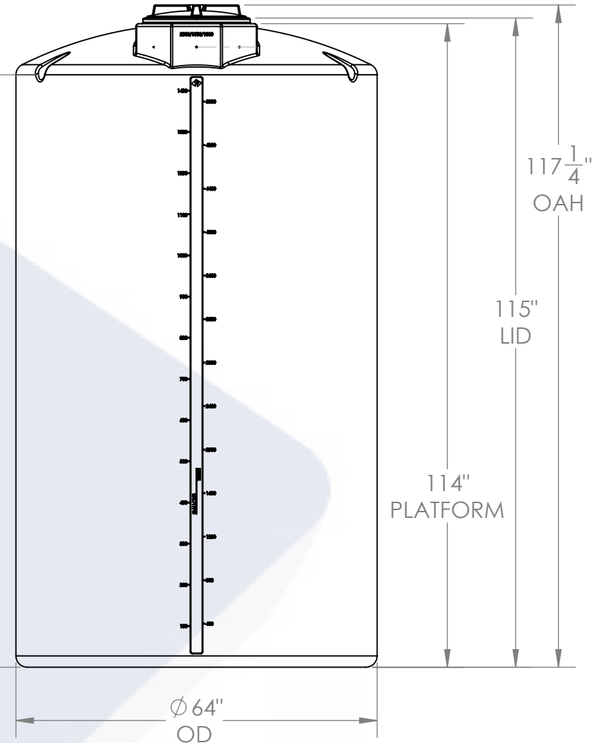
FRONT VIEW
