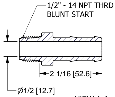
VIEW A-A SCALE 1 : 1
