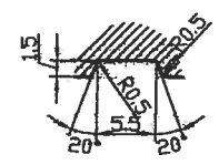
B-B SECTION SCALE=2:1
